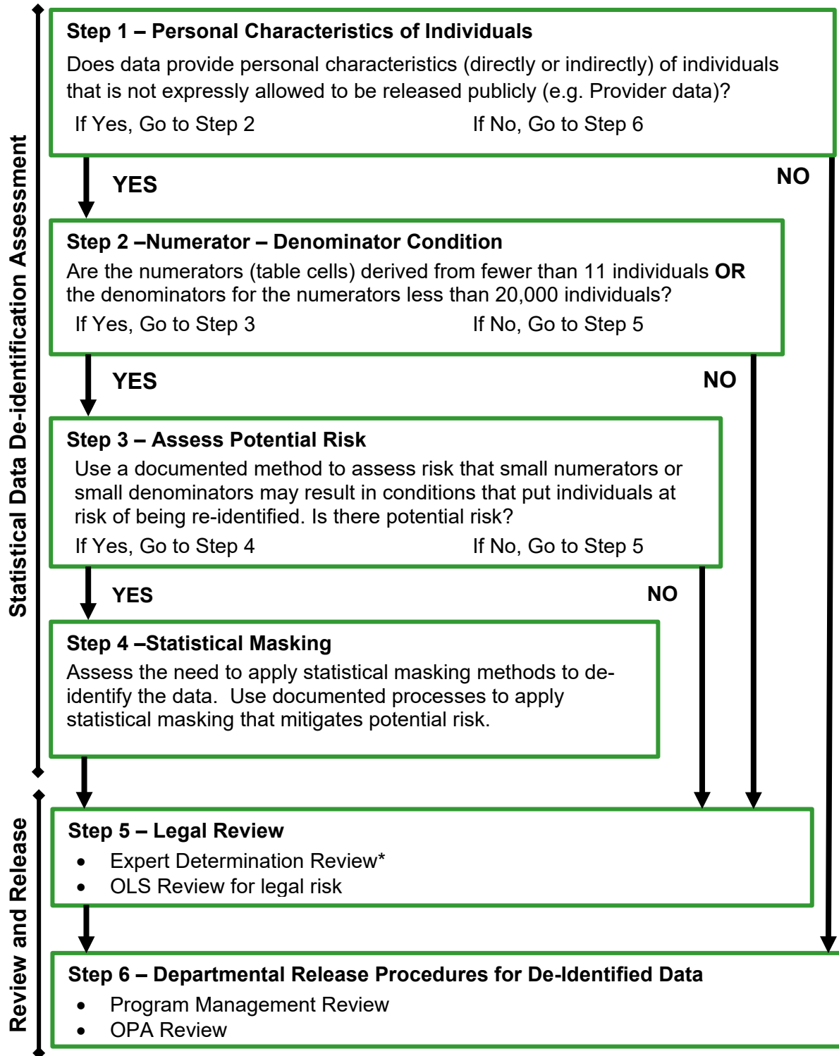
Figure 5: Data Assessment for Public Release Procedure
