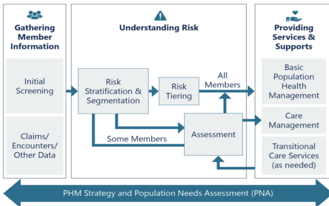
Figure 1. PHM Framework
